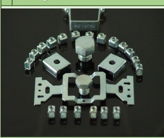
5.7 Zn coating on Steel
